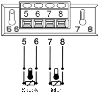
Fig.: Probe connection with 2 wire technology
